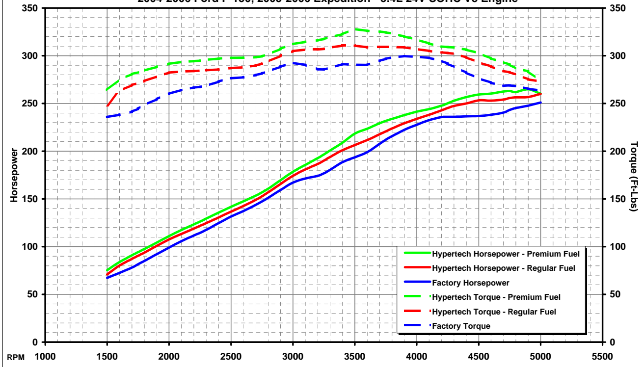
2004-2006 Ford F-150, 2005-2006 Expedition - 5.4L 24V SOHC V8 Engine
